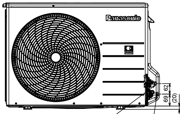
2-way valve at Liquid side (High Pressure)
